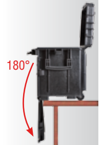
Front lid can be opened up to 180°
